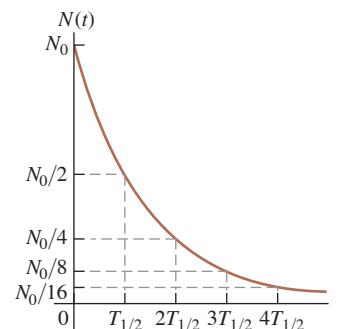
Figure 43.8 The number of nuclei in a sample of a radioactive element as a function of time. The sample's activity has an exponential decay curve with the same shape.
